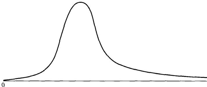
Figure 12.1 Lognormal distribution
